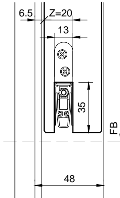
Typ: RDS17-48 38-41mm Türblatt
