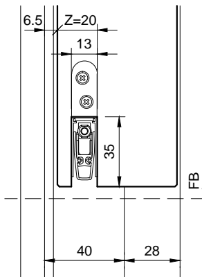
Typ: RDS17-28/40H,F 58-61mm Türblatt
